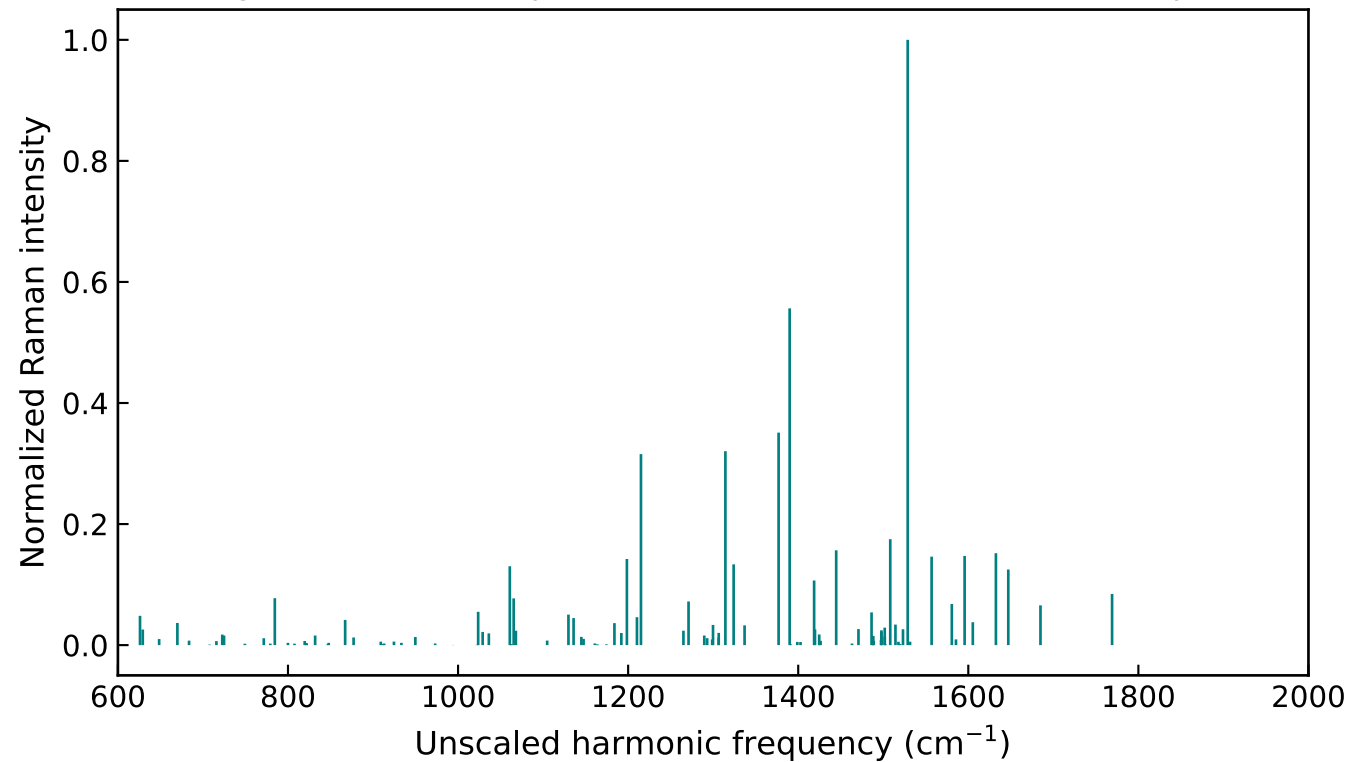
Figure 7. DFT stick spectrum (unscaled, B3LYP/6-311++G(d,p))
