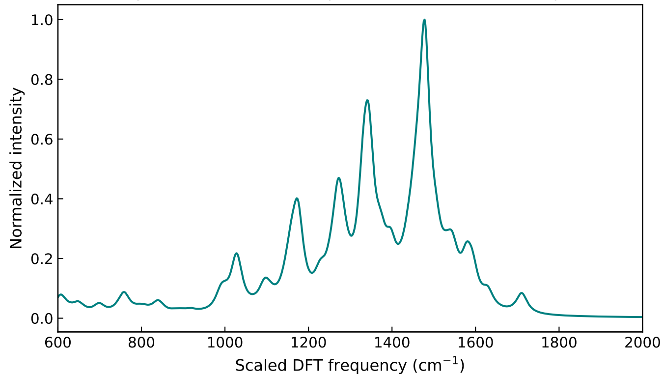
Figure 8. DFT broadened spectrum (Lorentzian line shape)
