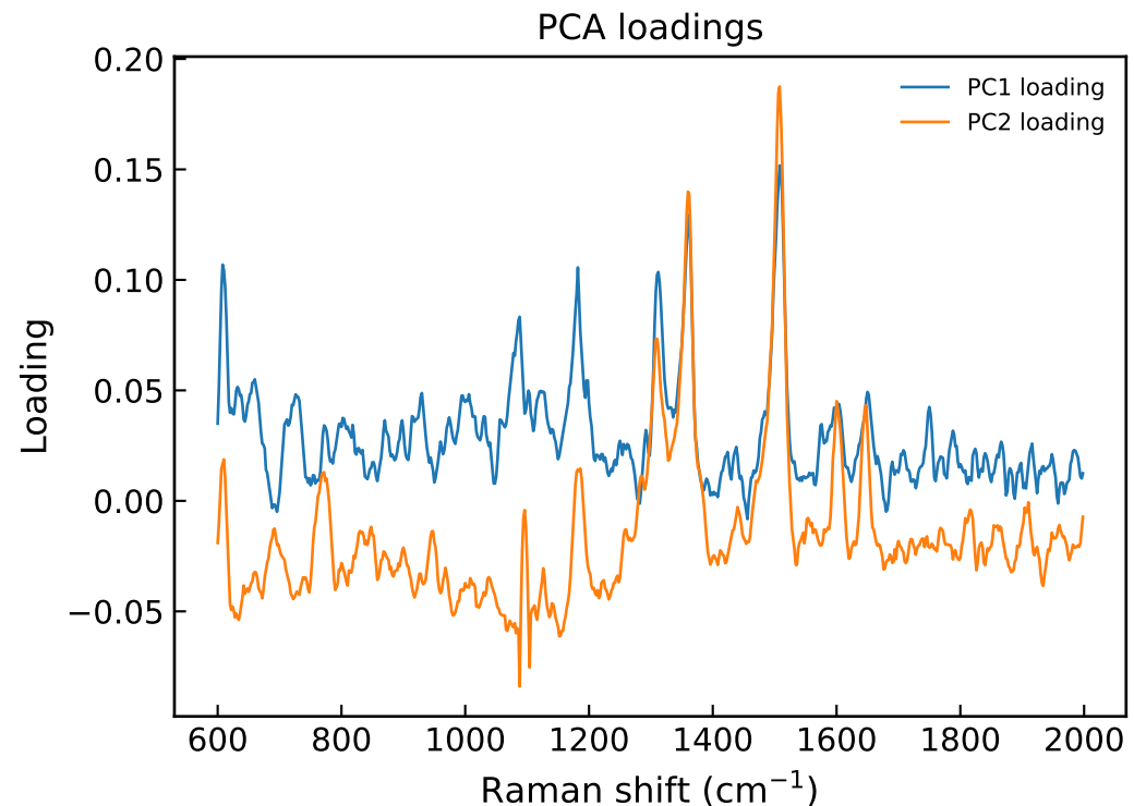
Figure 21. PCA of all 97 processed spectra
