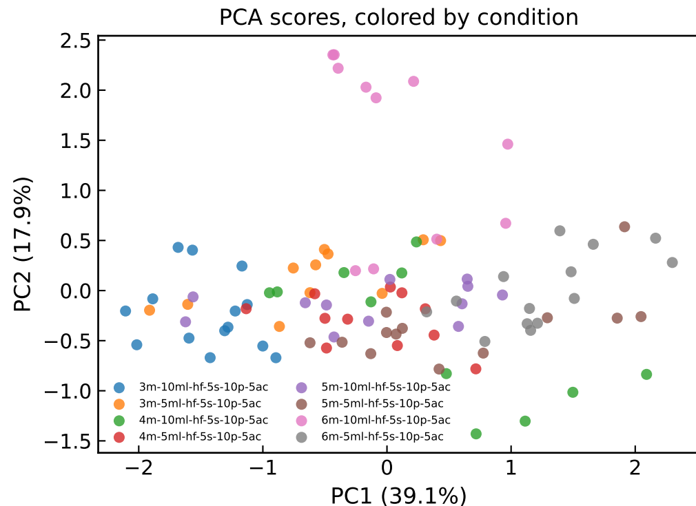
Figure 21. PCA of all 97 processed spectra
