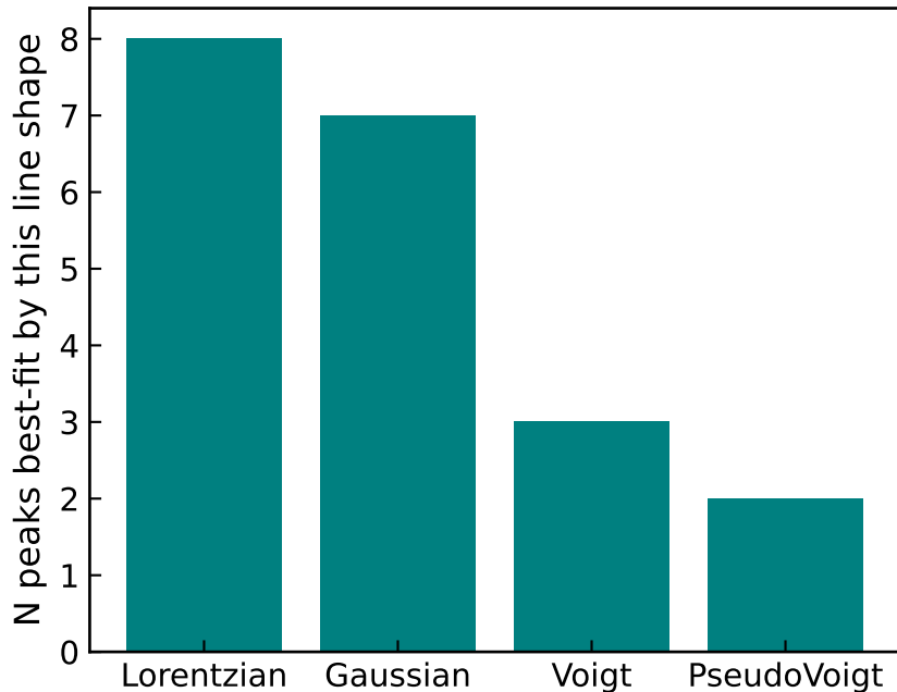
Figure 25. Best-fit line-shape distribution across fitted bands
