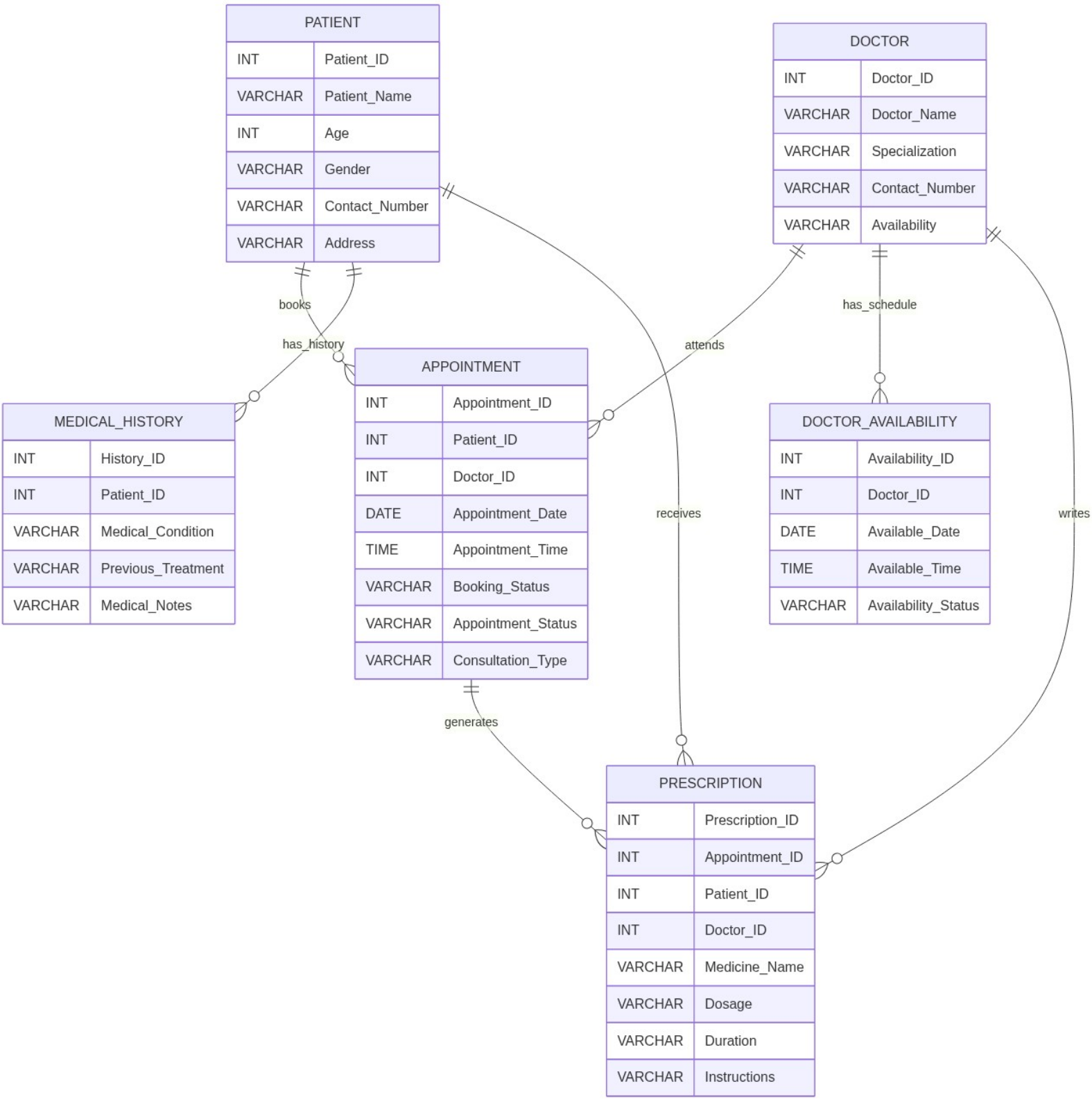
Medical Management System ER Diagram
