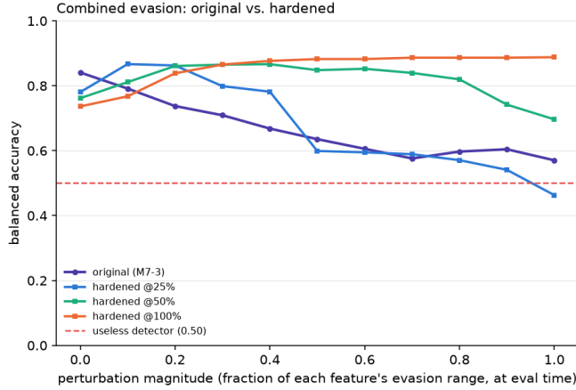
Fig. 6. Combined evasion (S VII's attack) against the original model and each hardened model.
