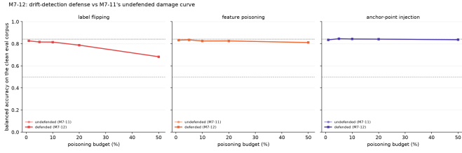
Fig. 18. Defended (Mahalanobis-gated) vs. undefended balanced accuracy, all three strategies, five budgets each.
