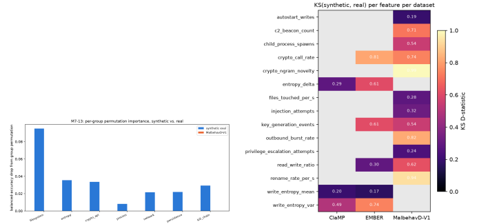
Fig. 12. Left: per-group permutation importance, synthetic eval vs. MalbehavD-V1 – every real bar is exactly zero. Right: KS D -statistic per feature per dataset (ClaMP/EMBER/MalbehavD-V1), the coverage-and-divergence pattern at a glance.
