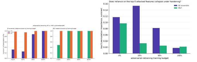
Fig. 10. Left: p10/median/p90 adaptive evasion by training budget, RF vs. MLP. Right: top-5 permutation-importance sum by training budget, RF vs. MLP.
