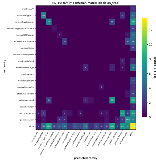
Fig. 13. 19×19 family confusion matrix, decision tree (the macro-F1 winner). Every row’s dominant off-diagonal mass sits in the white column – families are confused with benign, essentially never with each other.
