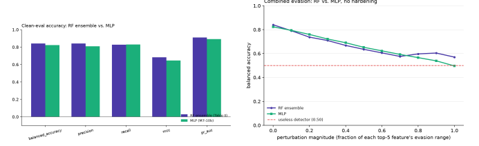
Fig. 8. Left: clean-eval accuracy, RF ensemble vs. MLP. Right: combined evasion, RF vs. MLP, no hardening.
