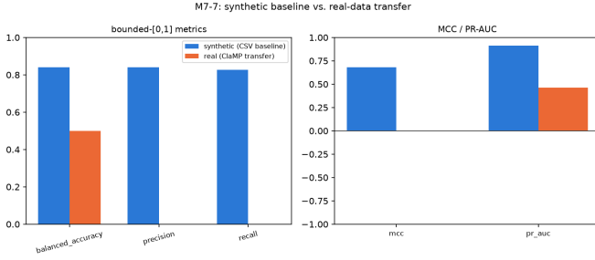
Fig. 9. Synthetic CSV-path baseline vs. ClaMP real-data transfer, same fitted ensemble.
