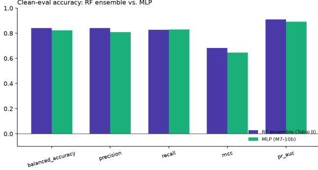
Fig. 11. Clean-eval accuracy, RF ensemble vs. MLP.
