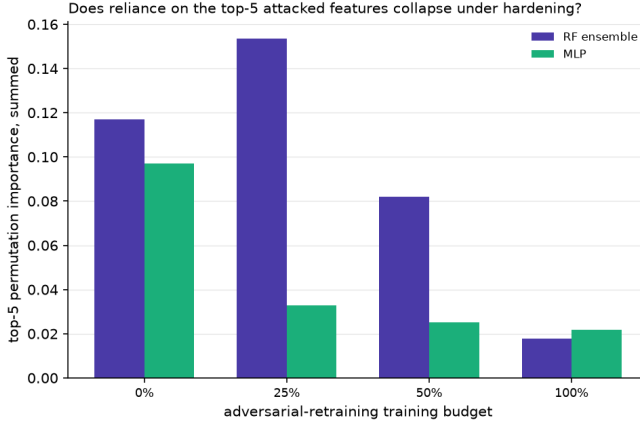
Fig. 14. Top-5 permutation-importance sum by training budget, RF vs. MLP.
