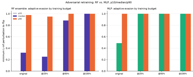
Fig. 13. p10/median/p90 adaptive evasion by training budget, RF vs. MLP.
