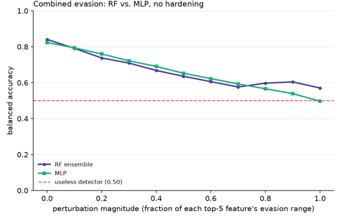
Fig. 12. Combined evasion, RF vs. MLP, no hardening.
