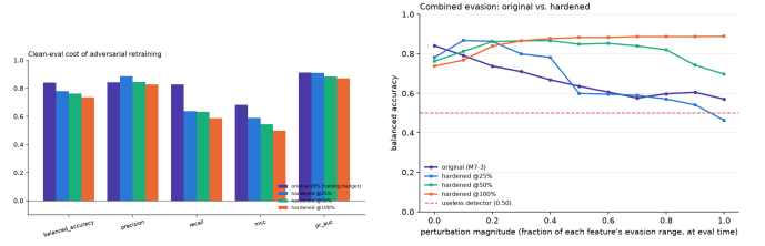
Fig. 6. Left: clean-eval metrics, original vs. hardened at each training budget. Right: combined evasion (§VI-B’s attack) against the original model and each hardened model.
