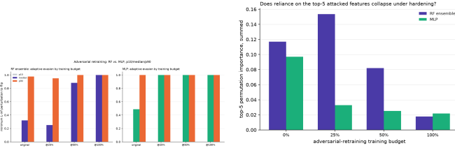
Fig. 10. Left: p10/median/p90 adaptive evasion by training budget, RF vs. MLP. Right: top-5 permutation-importance sum by training budget, RF vs. MLP.
