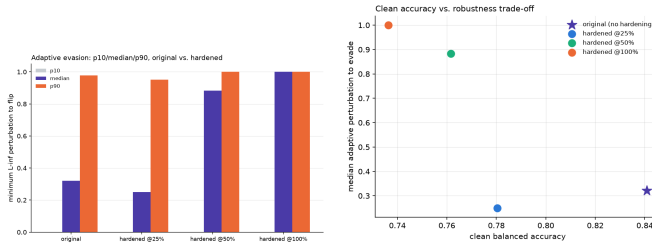
Fig. 7. Left: p10/median/p90 minimum perturbation to evade, original vs. each hardened budget. Right: clean balanced accuracy vs. median adaptive perturbation to evade – the deployment trade-off, one point per training budget.
