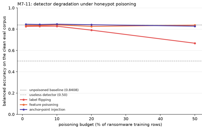
Fig. 17. Detector degradation under three poisoning strategies, five budgets each.
