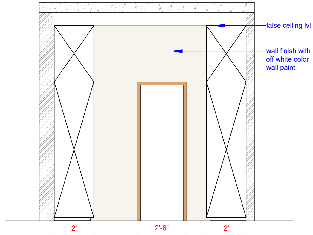
ELEVATION WALL C
