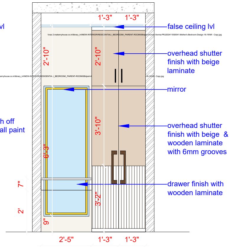
ELEVATION WALL B
