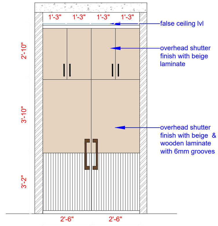
ELEVATION WALL D
