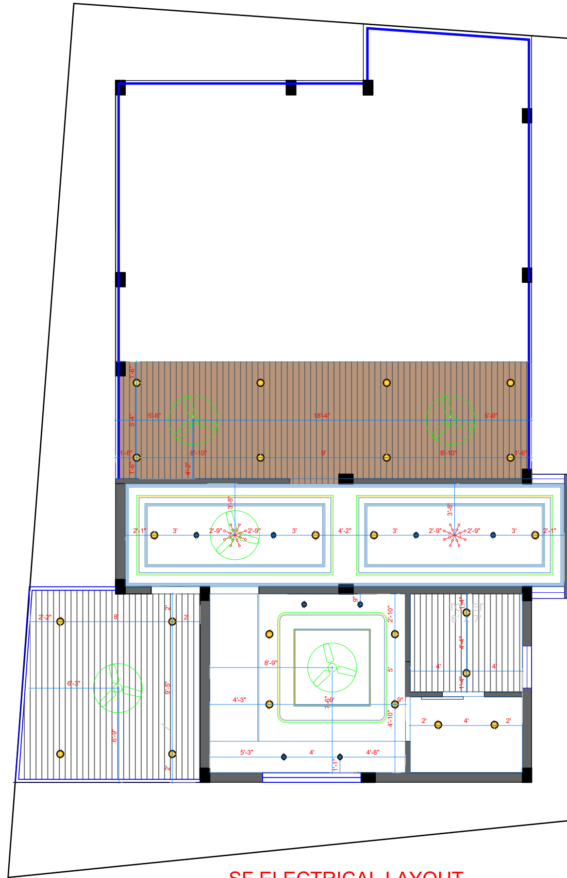
SF ELECTRICAL LAYOUT
