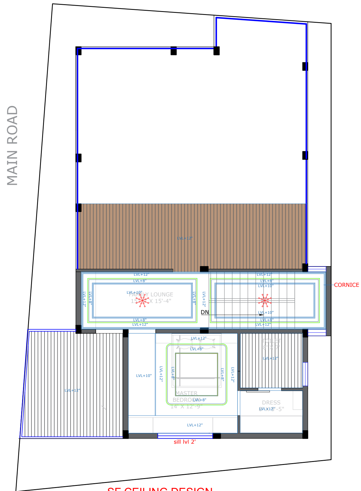
SF CEILING DESIGN FLOOR HT 11'6" INCLUDING SLAB
