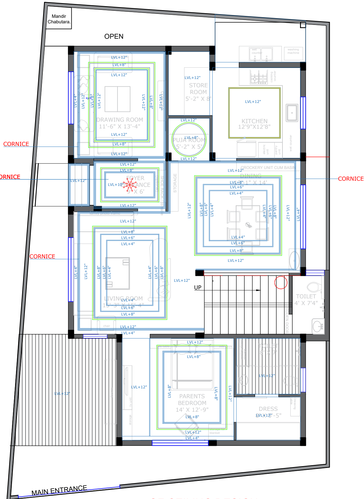
GF CEILING DESIGN
