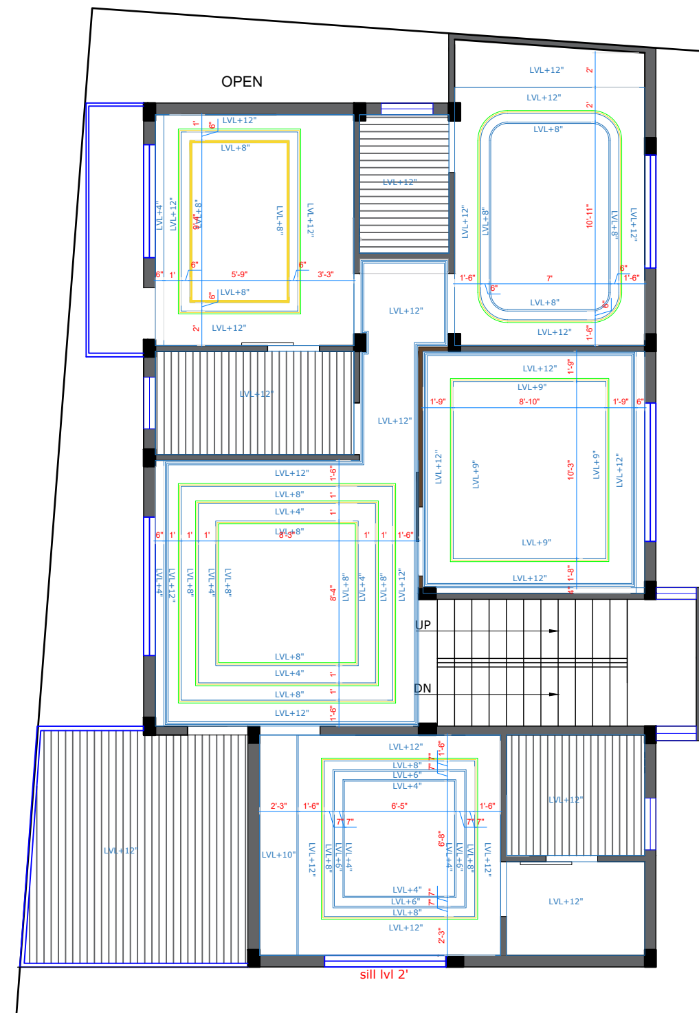
FF CEILING DETAIL
