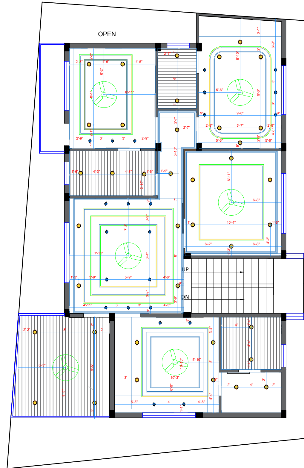
FF ELECTRICAL LAYOUT
