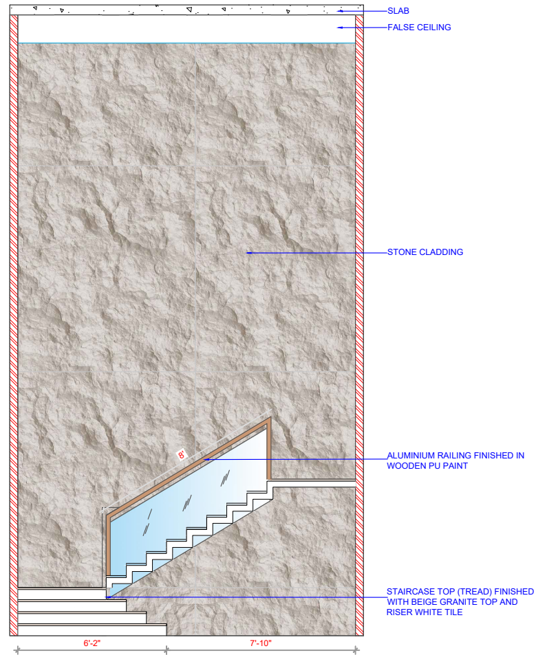
ELEVATION D
