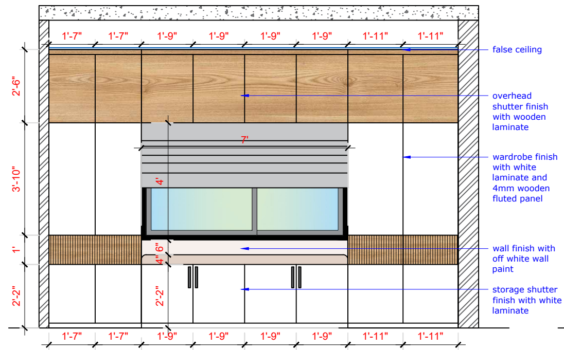
ELEVATION WALL - C
