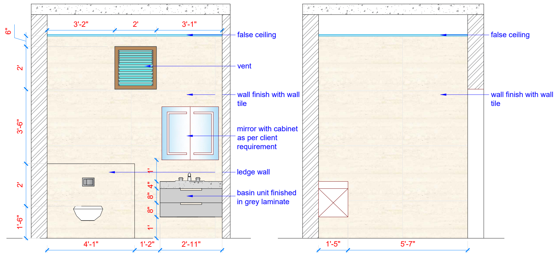
ELEVATION WALL - A
