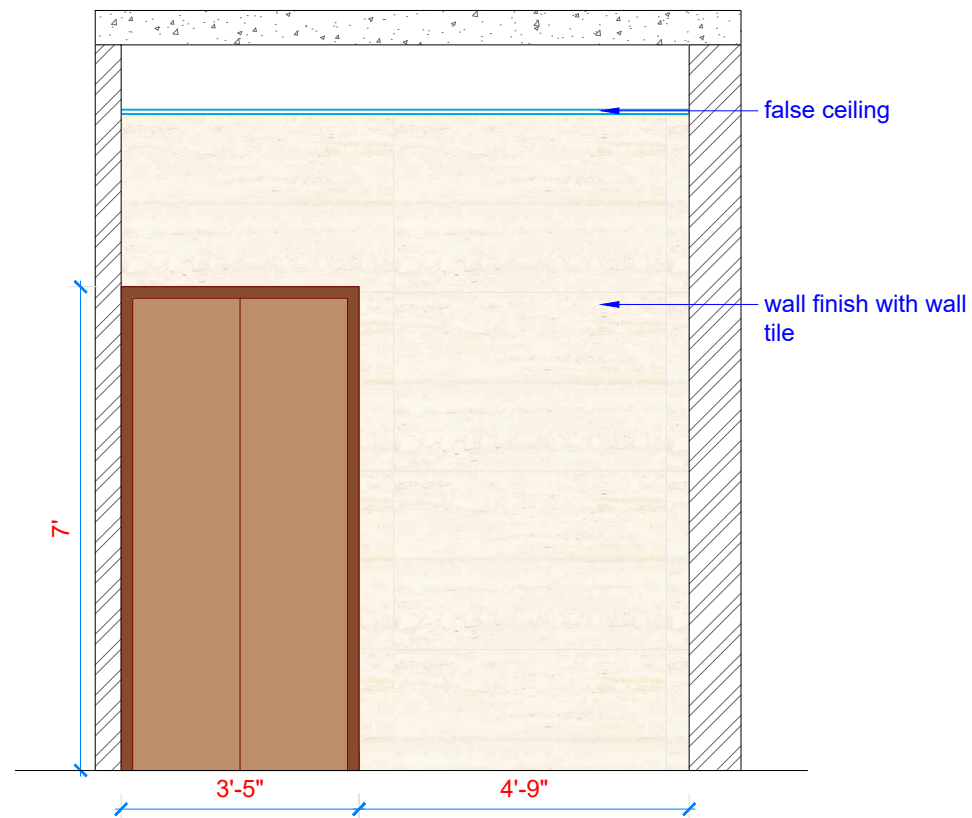
ELEVATION WALL - C
