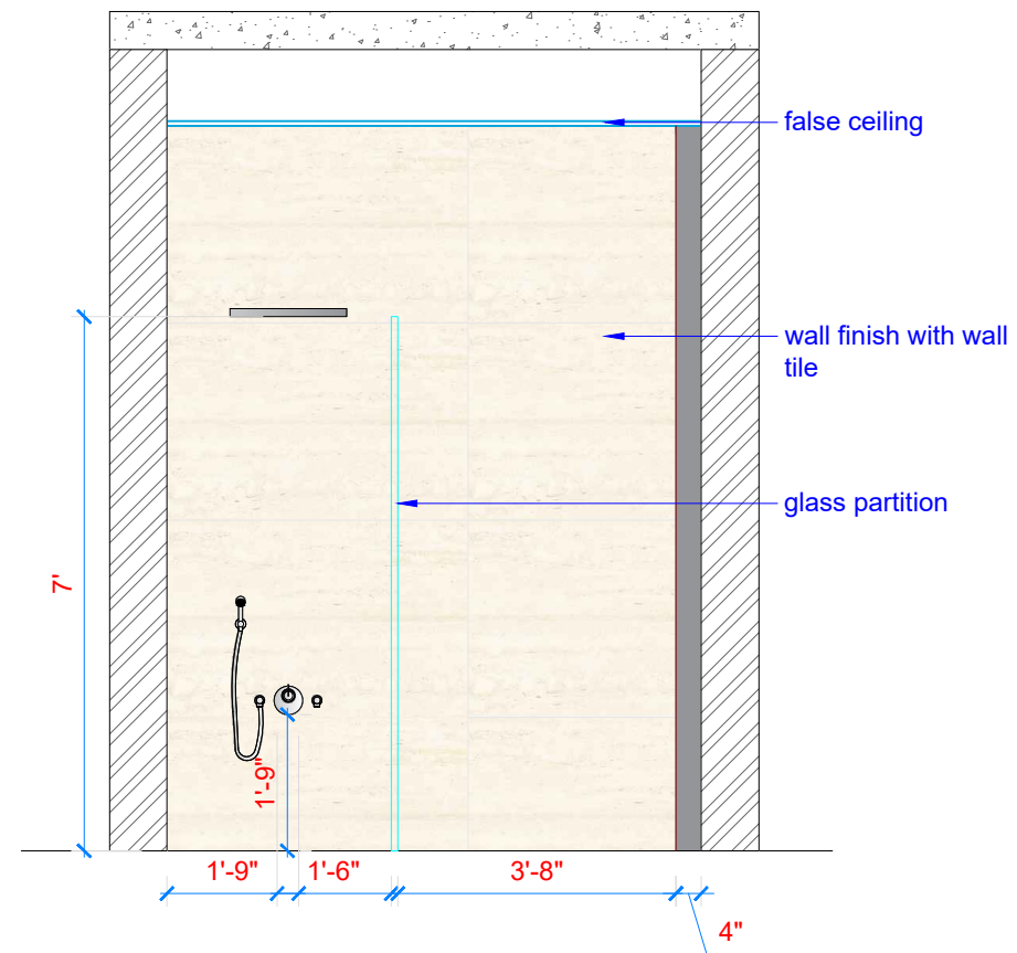
ELEVATION WALL - D
