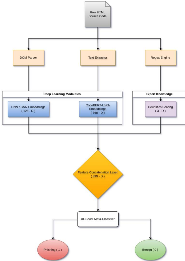
Fig. 2. The OmniPhish Tri-Modal Architecture detailing the parallel extraction of Spatial (CNN/GNN), Semantic (CodeBERT), and Heuristic features prior to XGBoost fusion.
