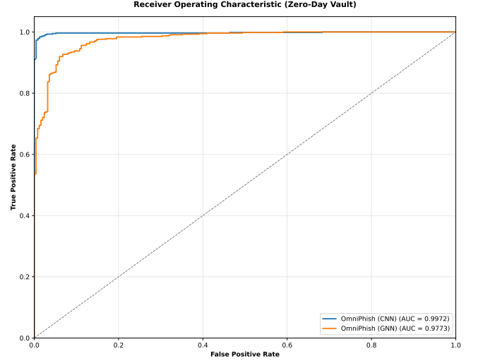
Fig. 4. Receiver Operating Characteristic (ROC) curve comparing the CNN and GNN variants against Zero-Day threats.
