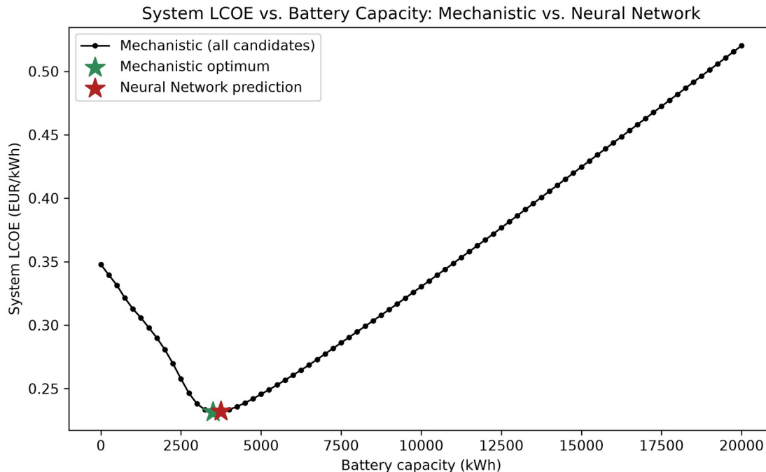
Figure 32 (full-scale, scenario 175) — System LCOE vs. battery capacity, mechanistic sweep with the mechanistic optimum (green star) and neural network prediction (red star) marked. The two stars sit almost on top of each other at the curve's minimum.
