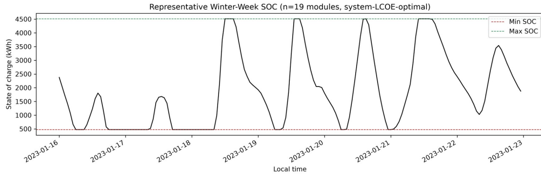
Figure 10 — SOC trajectory for the system-LCOE-optimal battery (19 modules), a representative winter week.
