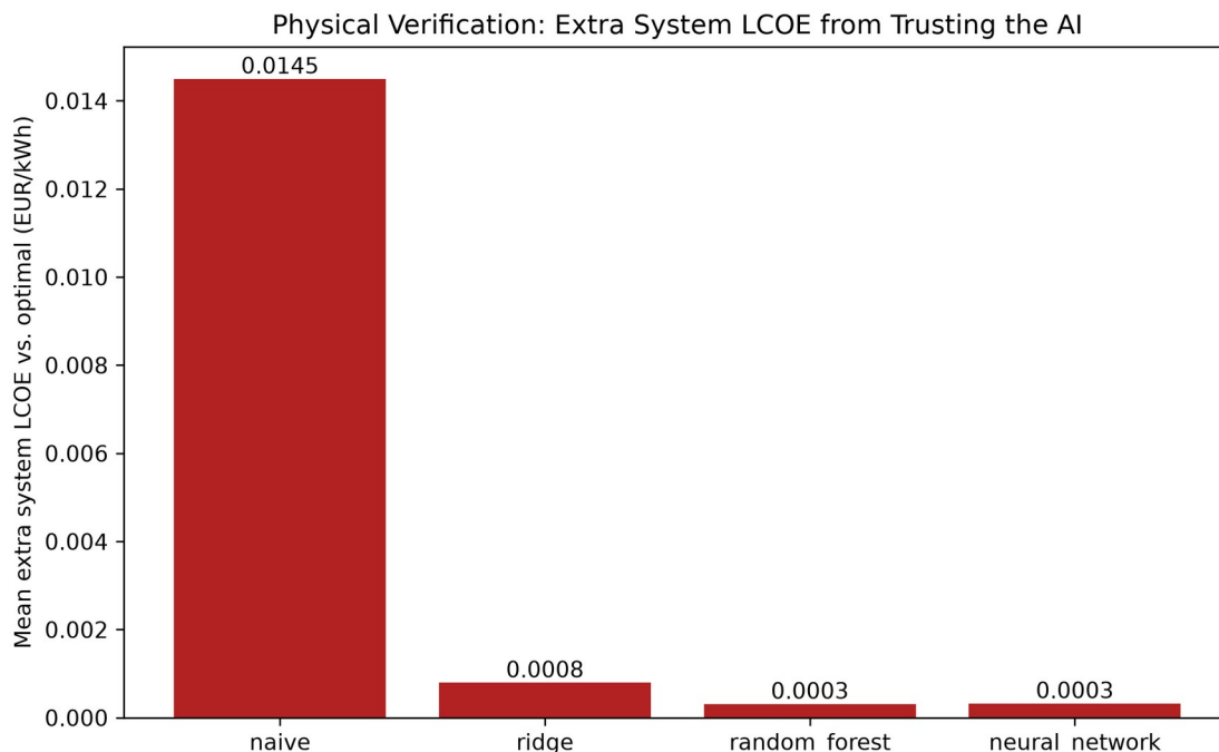
Figure 29 (full-scale) — Mean extra system LCOE by model, clean
