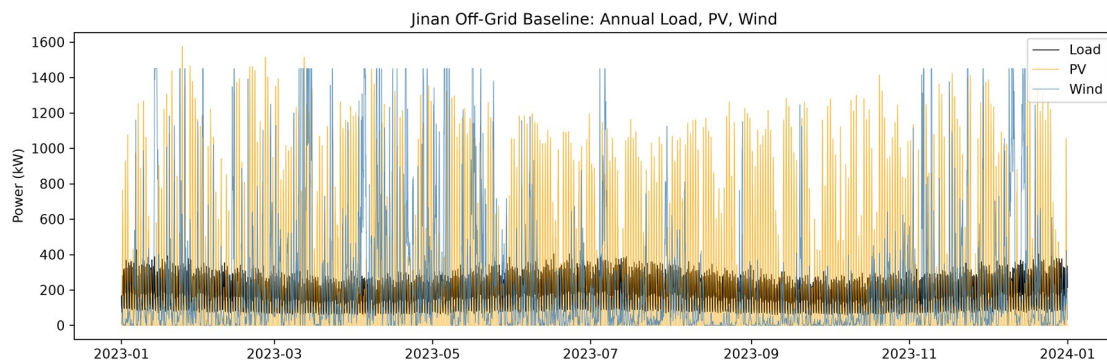
Baseline off-grid annual load, PV, and wind profile (Jinan, 2023)
