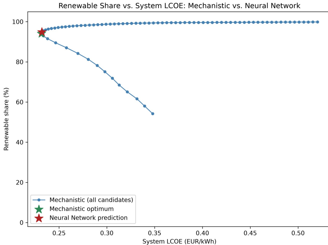
Figure 33 (full-scale, scenario 175) — Renewable share vs. system LCOE, mechanistic sweep with the mechanistic optimum (green star) and neural network prediction (red star) marked. The two stars sit almost on top of each other at the curve's elbow.
