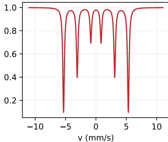
Sexteto (BHF = 33 T)
