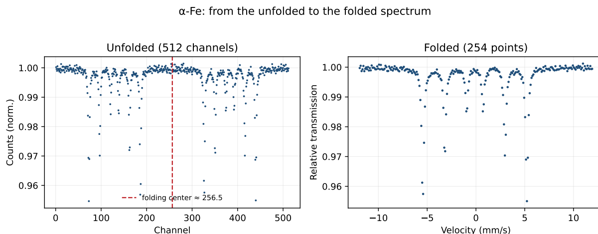
Figure 3.1: The same \alpha -Fe unfolded (left, 512 channels) and folded (right, in velocity). Unfolded, the transducer measures the sextet twice —once in each branch of the sweep— mirrored about the folding centre (red line). Folding sums those two halves: it reduces the noise and produces the symmetric spectrum on the right.
