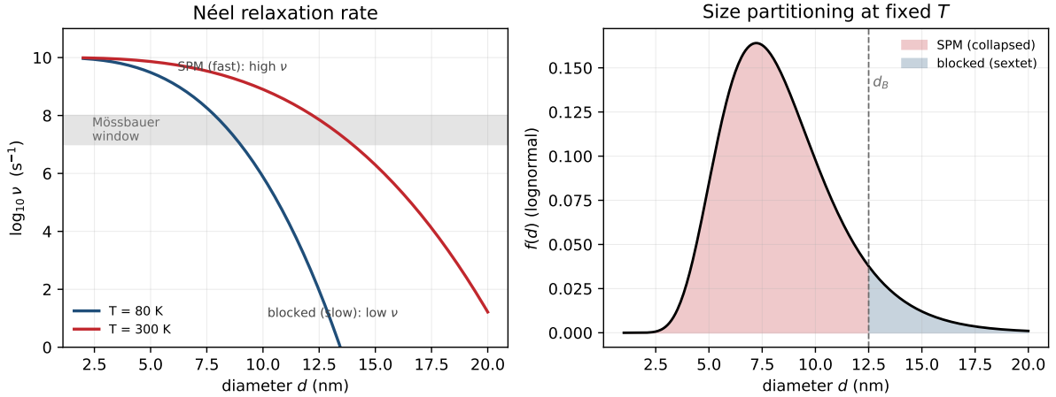
Figure E.3: Néel-Arrhenius: size-dependent blocking. Left : the relaxation rate \nu(d, T) drops as the diameter grows; small particles relax fast (superparamagnetic, collapsing to a singlet/doublet) and large ones remain blocked (sextet). A particle appears blocked when \nu falls below the Mössbauer observation window (grey band); as T decreases the blocking shifts to smaller diameters. Right : over a lognormal size distribution, at fixed T the blocking diameter d_B separates the superparamagnetic fraction from the blocked one, and the spectrum is the mixture of both.
