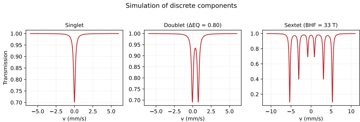
Figure 4.1: Simulation of the three discrete components: singlet (one peak), doublet ( \Delta E_Q = 0.80 mm/s) and sextet ( B_{\text{hf}} = 33 T with intensity ratio 3 : 2 : 1).
