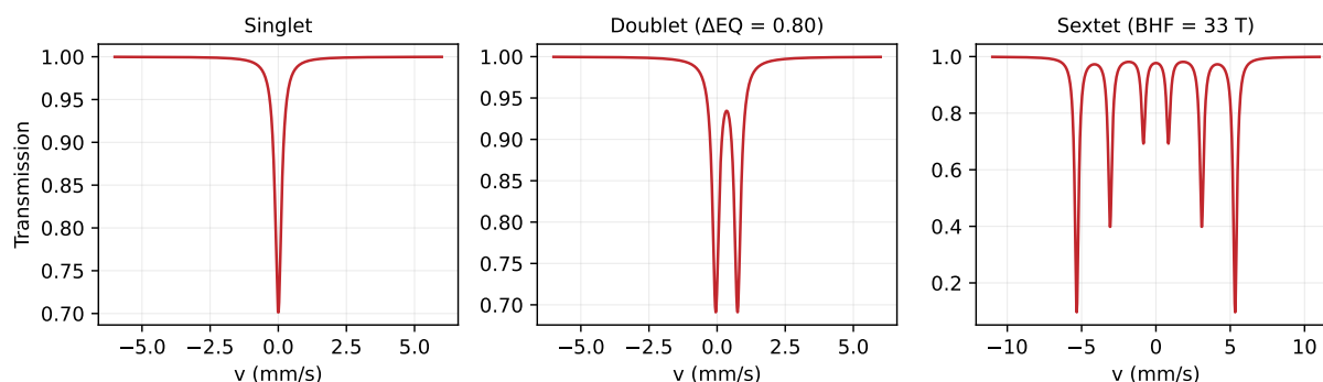
Figure 4.1: Simulation of the three discrete components: singlet (one peak), doublet ( \Delta E_Q = 0,80 mm/s) and sextet ( B_{\text{hf}} = 33 T with intensity ratio 3 : 2 : 1).
