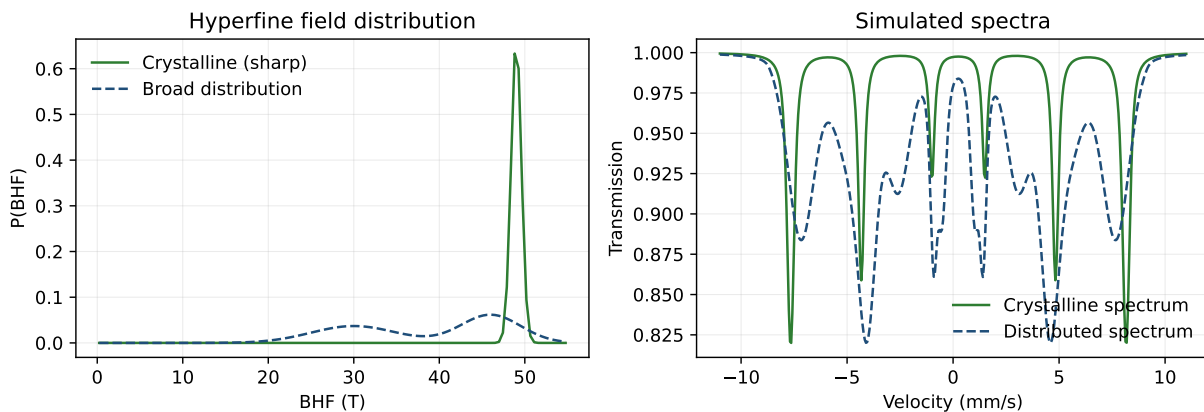
Figure 5.1: Left: crystalline hyperfine field distribution (sharp, around 49 T) versus a broad distribution. Right: the corresponding simulated spectra. The broad distribution “blurs” and overlaps the sextet lines.
