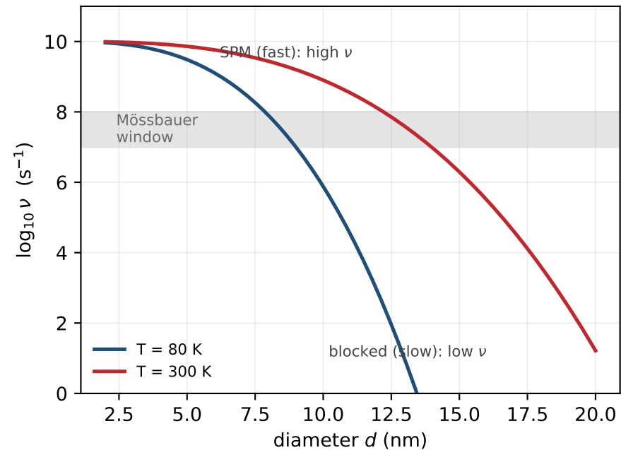
Néel relaxation rate
