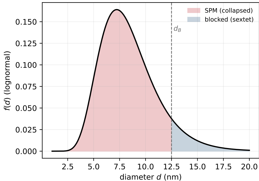
Size partitioning at fixed T
