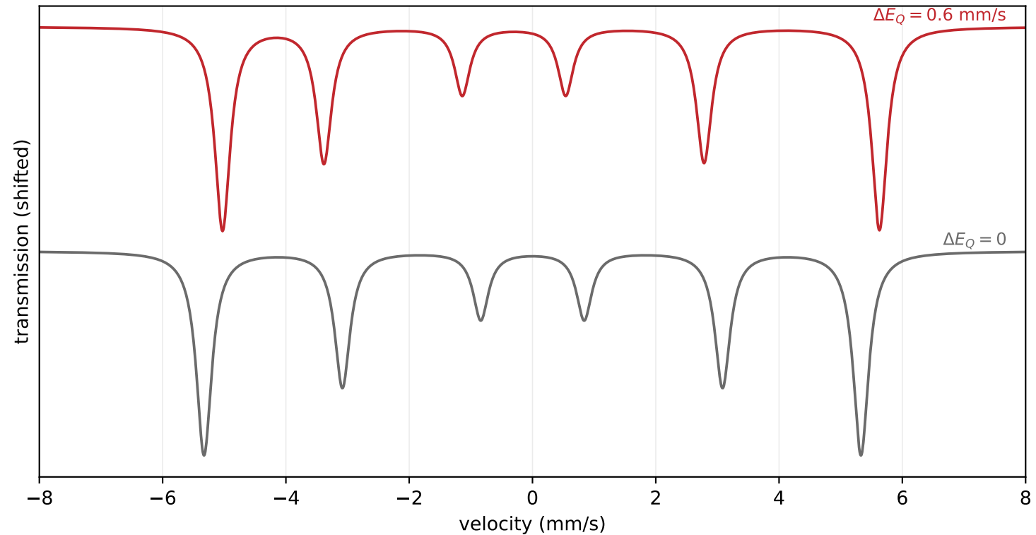
Effect of the quadrupole on a sextet (first order)
