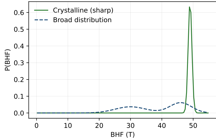
Hyperfine field distribution
