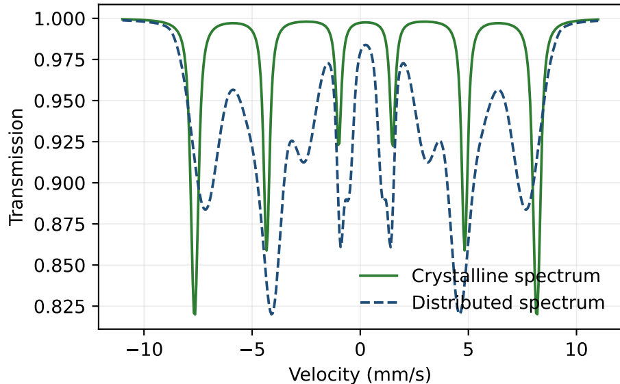
Simulated spectra
