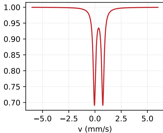
Doublet ( \Delta EQ = 0.80 )
