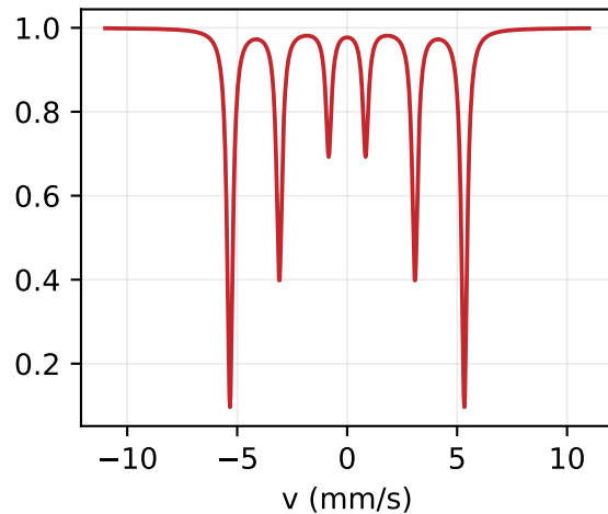
Sextet (BHF = 33 T)
