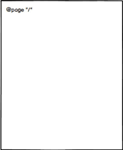
Home.razor
