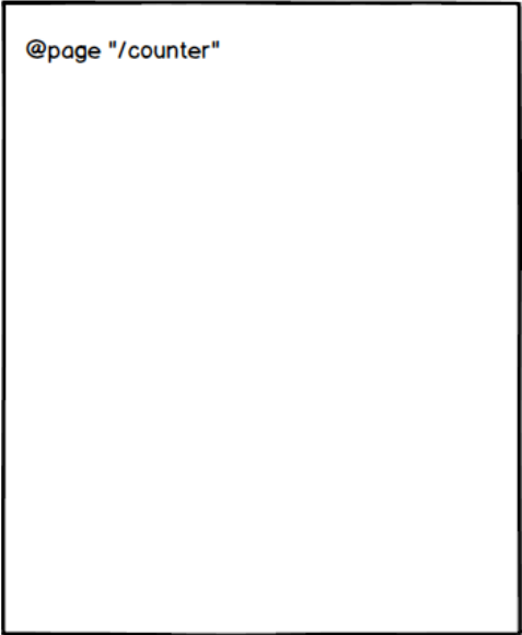
Counter.razor
