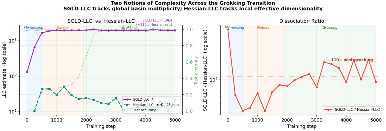
Figure 2. Local flatness and global multiplicity diverge at grokking. Left: SGLD-LLC (purple, sensitive to global multiplicity) and Hessian-estimated LLC \hat{\lambda}_H (teal, sensitive to local flatness) on a shared log axis, with test accuracy (green dots). Both are high during memorisation; at the grokking transition \hat{\lambda}_H collapses while SGLD-LLC stays elevated—two orders of magnitude apart post-grokking. The value \hat{\lambda}_H \approx 18 matches the intrinsic dimensionality of the Fourier circuit ( \sim 12 frequencies \times 2 parameters). Right: Ratio of the two estimators over time. The ratio jumps at the grokking transition and remains elevated—a geometry-based phase detector that requires no labelled test set.
