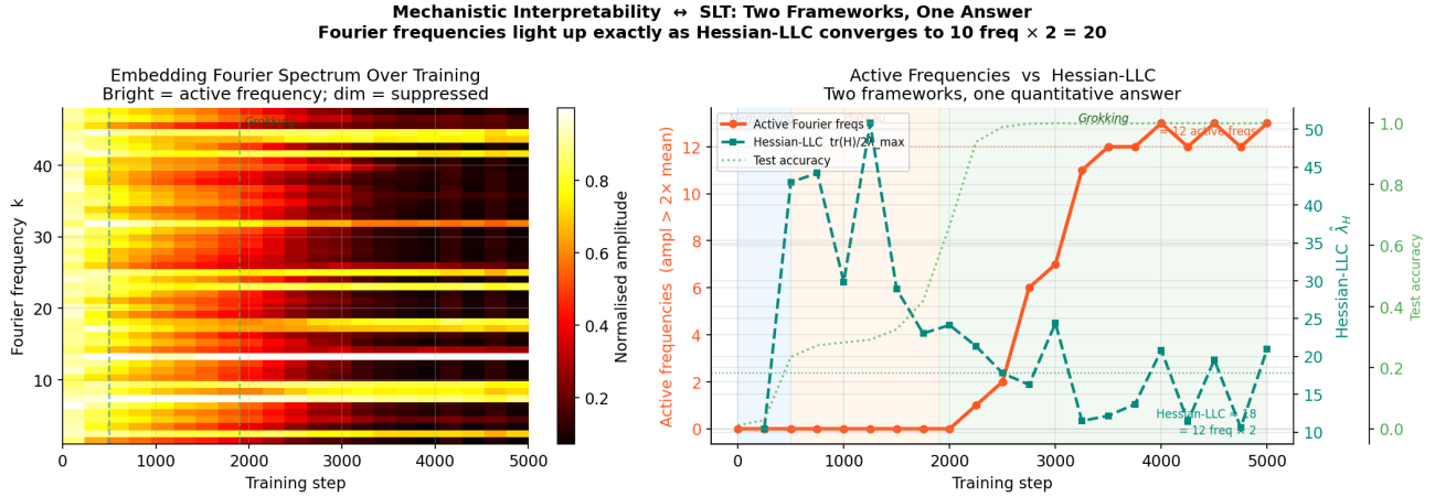
Figure 3. Circuit Imprint: loss-geometry independently recovers the circuit’s dimensionality. Left: Token-embedding Fourier spectrum across training (bright = high amplitude). Through the memorisation phase all frequencies are dim and equal; at the grokking transition a small set abruptly activates (vertical green dashed line) while others remain near zero. Right: Active frequency count (orange) and \hat{\lambda}_H (teal) both transition at the same training step and reach consistent values post-grokking. The two signals are derived from entirely different objects (embedding spectrum vs. loss-surface curvature) and share no information, yet converge simultaneously.
