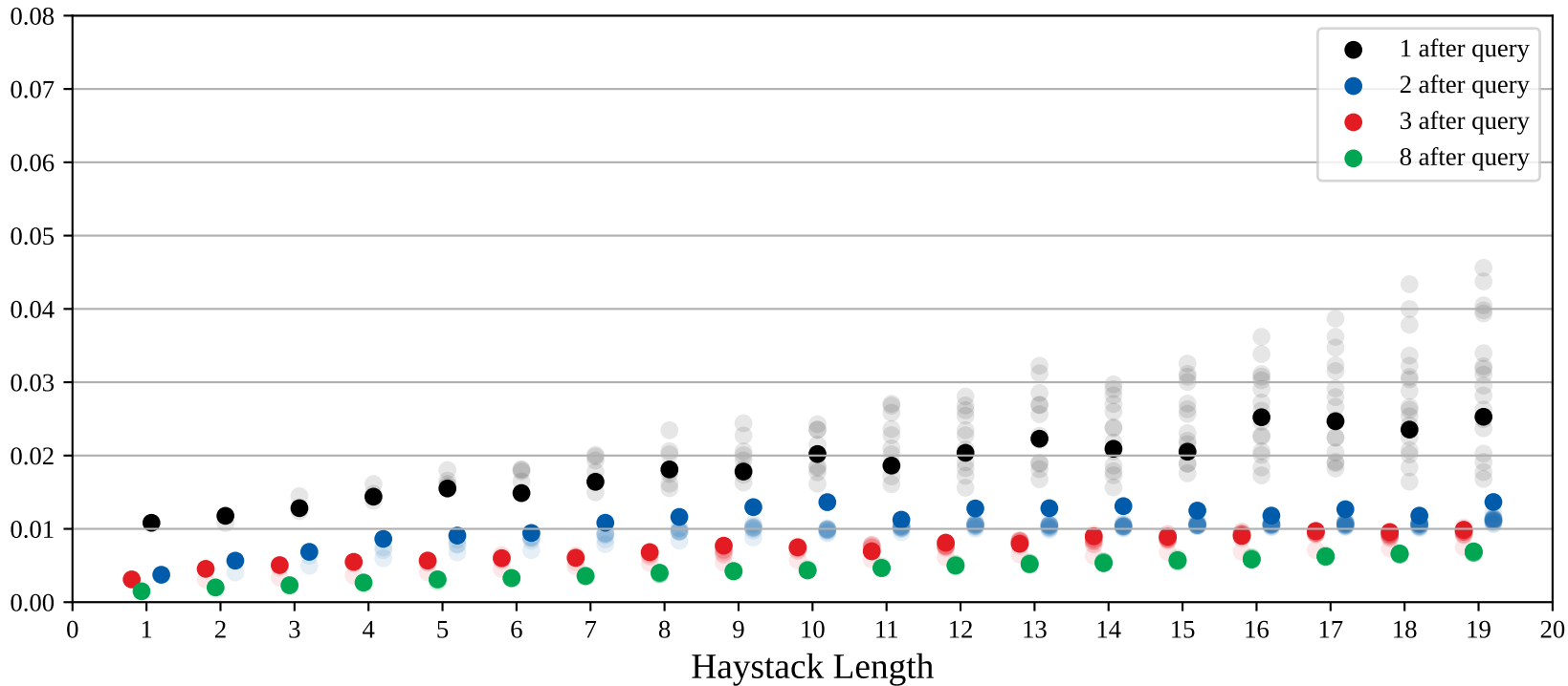
Error after 6.25e7 Training Traces
