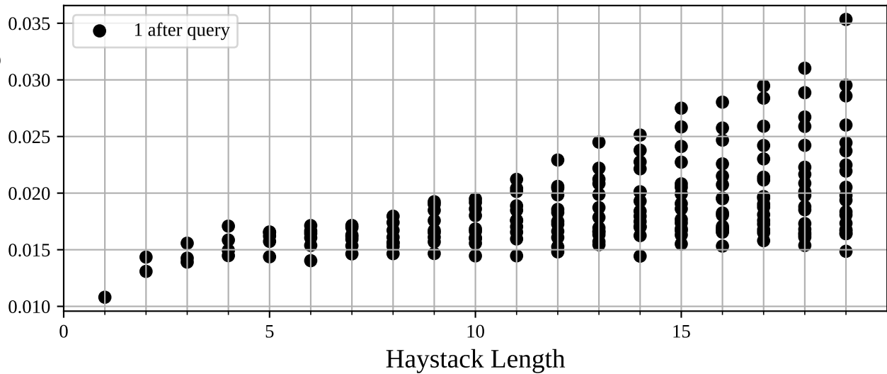
Error after 6.25e7 Training Traces
