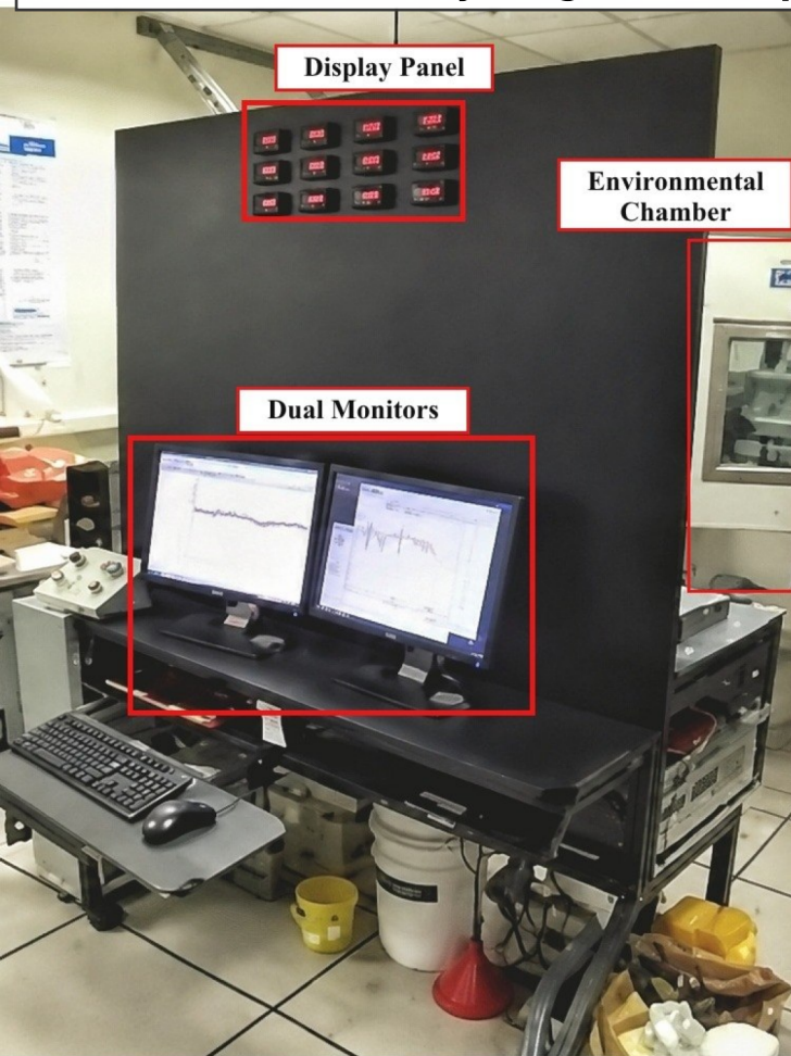
(a) NASA Ames Battery Prognostics Experimental Platform
