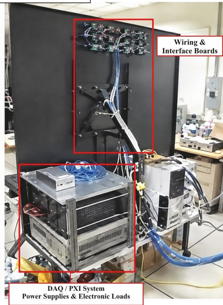
(a) NASA Ames Battery Prognostics Experimental Platform
