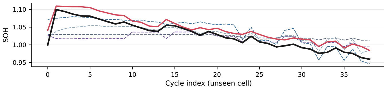
(c) B0032 — unseen cell
