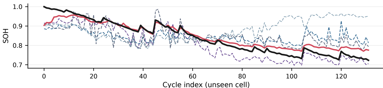
(b) B0018 — unseen cell
