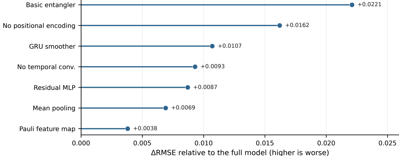
Architectural component ablation on NASA
