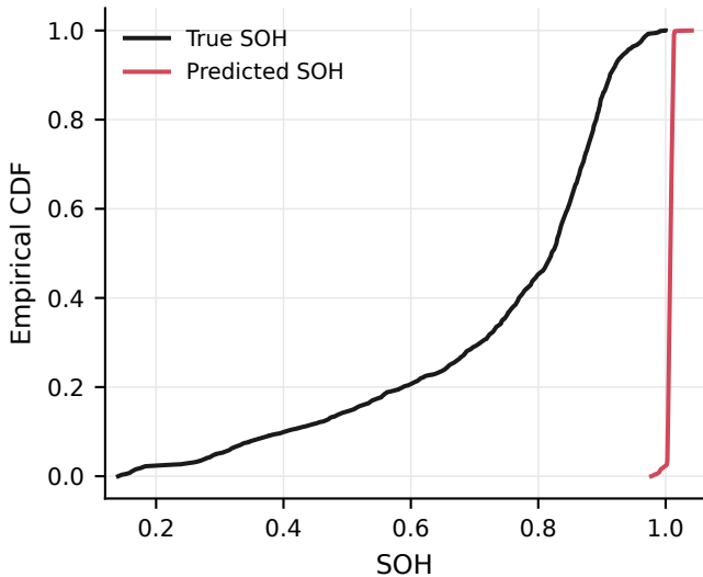
Pooled SOH distribution mismatch
