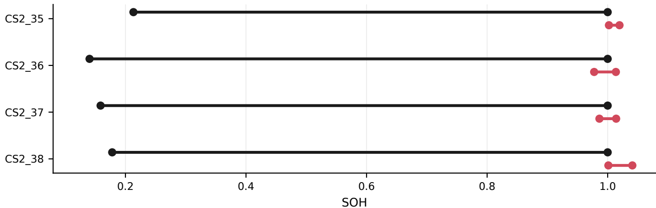
True versus predicted SOH range by cell
