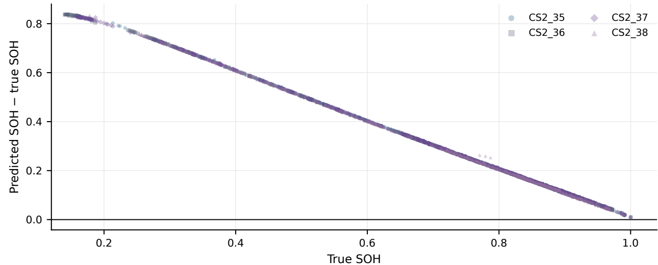
Residual versus true SOH under zero-shot transfer
