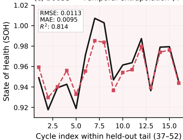
(c) B0053 — Temporal extrapolation (4 °C)
