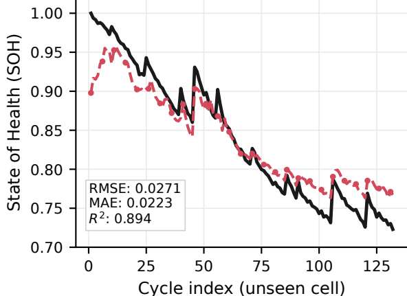
(c) B0053 — Temporal extrapolation (4 °C)
