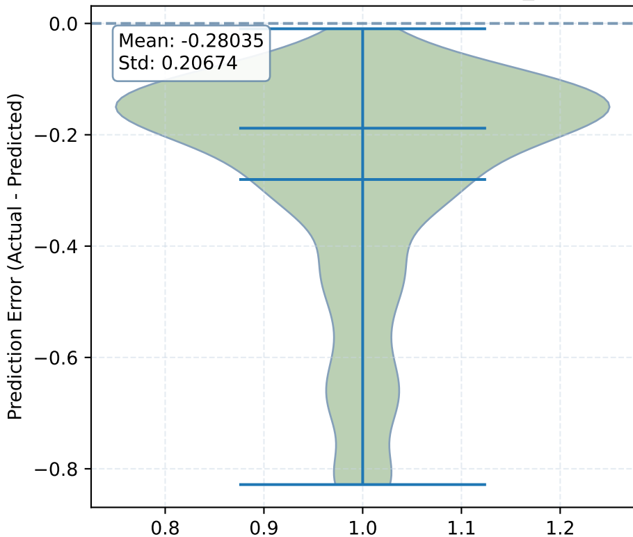
Prediction Error Distribution (CS2_37)
