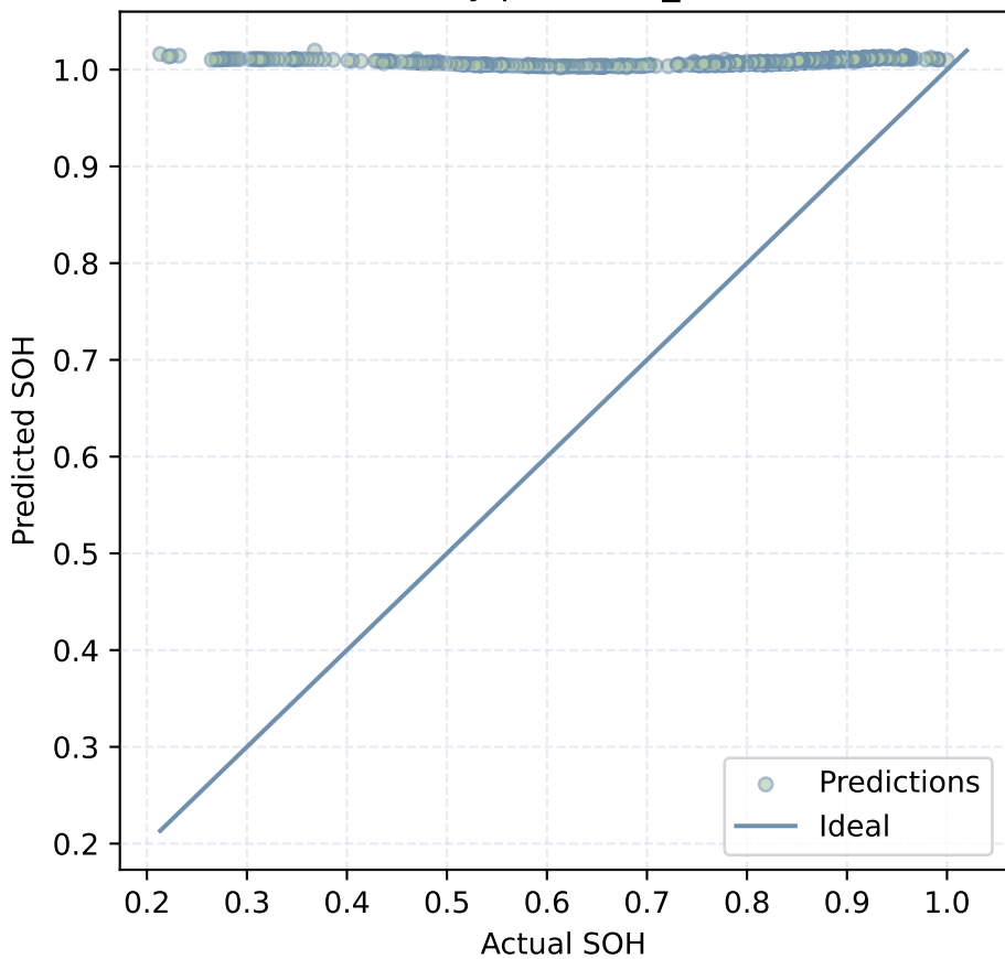
Parity plot (CS2_35)
