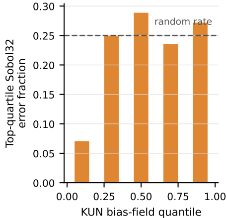
b Difficulty enrichment
