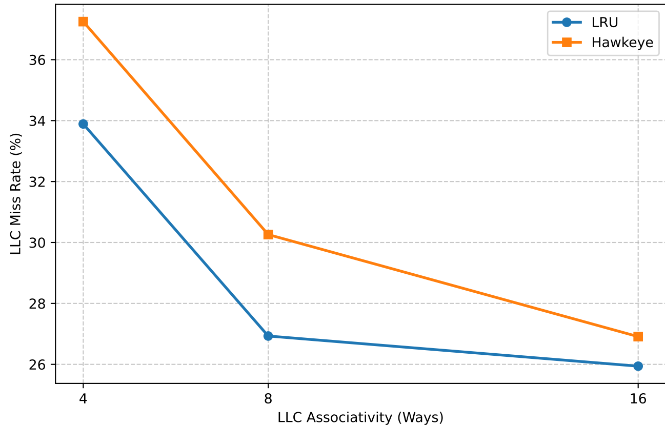
LLC Miss Rate vs. Associativity (456.hmmer-191B)
