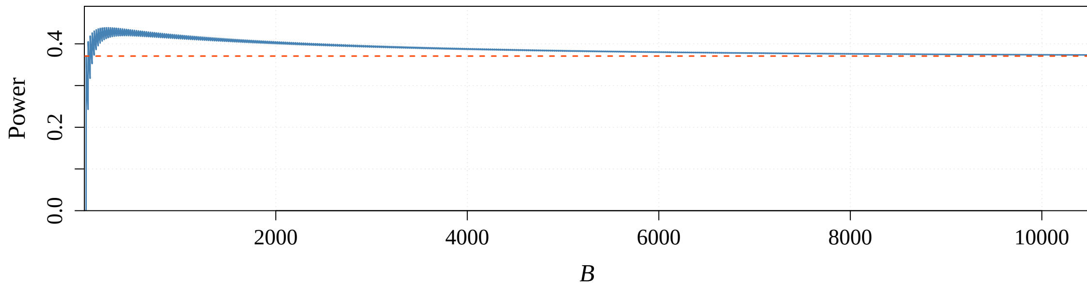
Case 2 ( n = 25 )
