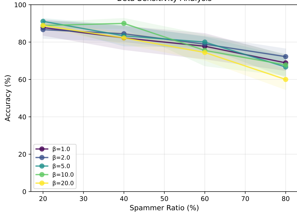
Beta Sensitivity Analysis
