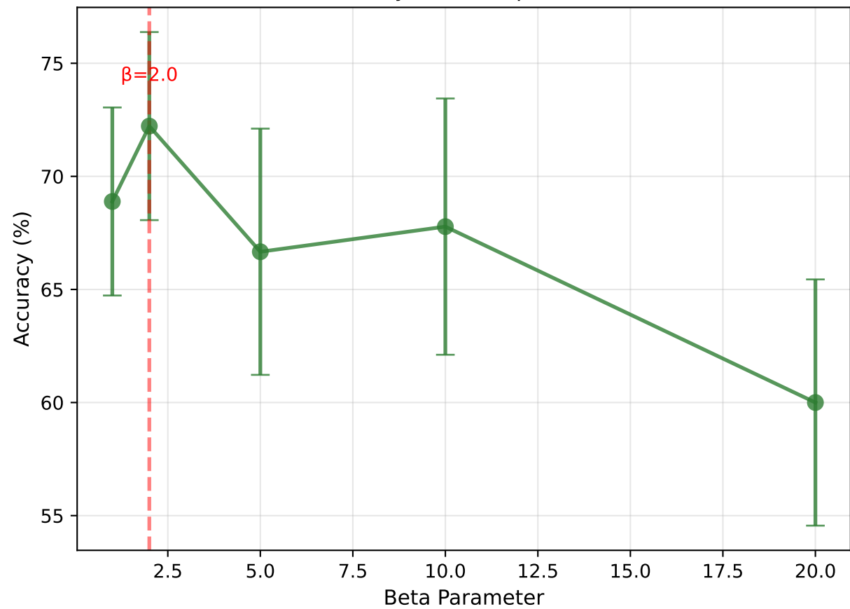
Accuracy at 80% Spammers
