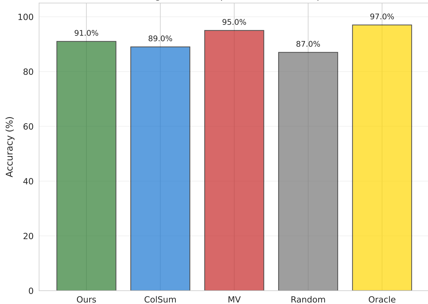
Track B: Algorithm Comparison (Natural Experiment)
